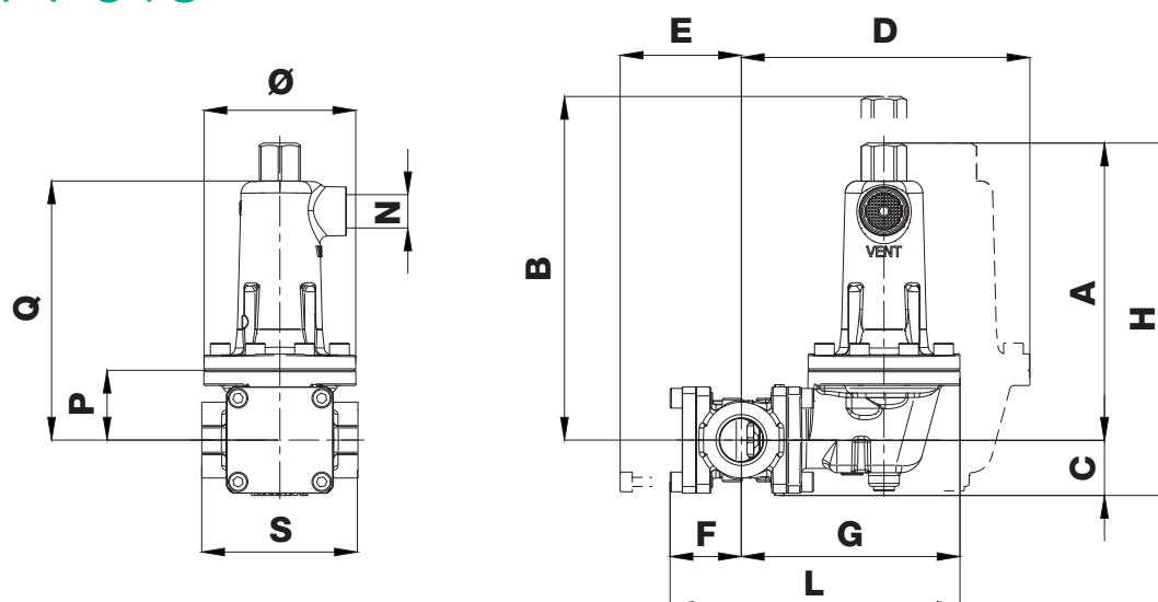
Figure 10 FT 518 dimensions
